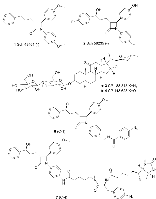
Figure 1. Structures of known cholesterol absorption inhibitors ( 1–4 ) and structures of two photoreactive analogous 2-azetidinones ( C-1 and C-4 ).
