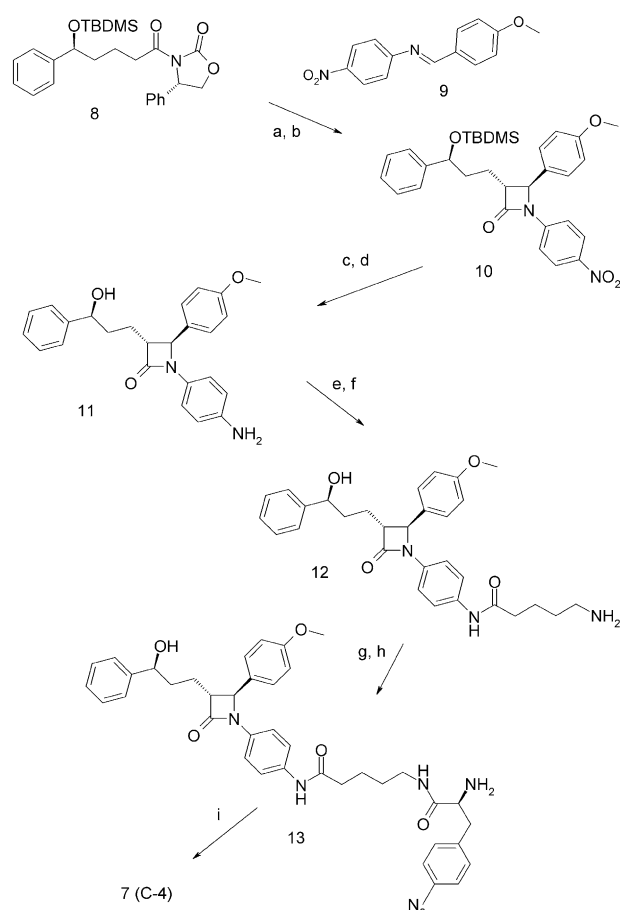
Scheme 1. Synthesis of biotin-labeled photoaffinity probe C-4 : (a) DIPEA, TMSCl, TiCl 4 , CH 2 Cl 2 (74%); (b) BSA, MTB-ether, TBAF (cat) (70%); (c) H 2 , Pd/C, 2 h, 5 bar, ethyl acetate (86%); (d) aqueous 2 N HCl, THF, 2 h, rt; (e) 5-(Fmoc-amino)-valerianic acid, TOTU, ethyl (hydroxyimino)-cyanoacetate, NEM (all from Fluka), DMF, 1 h, rt (41%); (f) NHEt 2 , DMF, 1 h, rt (56%); (g) Fmoc- p -azido-Phe-OH (Bachem), TOTU, ethyl (hydroxyimino)-cyanoacetate, NEM (all from Fluka), DMF, 1 h, rt (82%); (h) NHEt 2 , DMF, 1 h, rt (19%); (i) D-biotin- N -succinimidyl ester (Bachem), DMF, 1 h, rt (55%).
