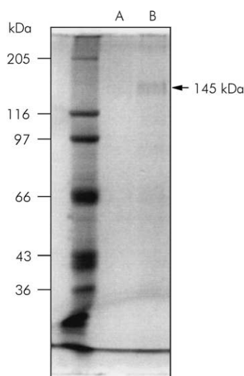
Figure 2. Photoaffinity labelling of rabbit ileal brush border membrane vesicles with C-4 and following streptavidin–biotin extraction. 200 \mu g of rabbit ileal brush border membrane vesicles were incubated with 200 \mu M of photoaffinity probe C-4 without (A) or with UV-irradiation (B). After solubilisation of membrane proteins, the proteins containing the biotin-tagged cholesterol absorption inhibitor C-4 were extracted with streptavidin–agarose beads. Bound proteins were released with 6 mM biotin and subsequently analysed by SDS-gel electrophoresis and staining with Coomassie-Blue R-250.
